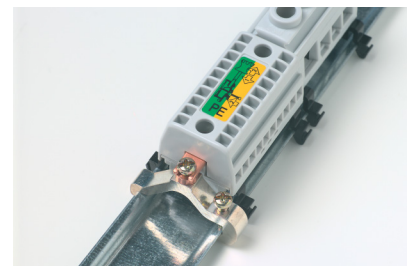
The markings serve as a reminder that the wire entry in the terminals must always be opened with a tool, e.g. a screwdriver - a good contact is thus guaranteed even in extreme conditions. Faulty installation is prevented by the design of the terminal.
